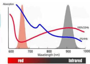
Absorption Spectrum for Oximeter on 660nm
